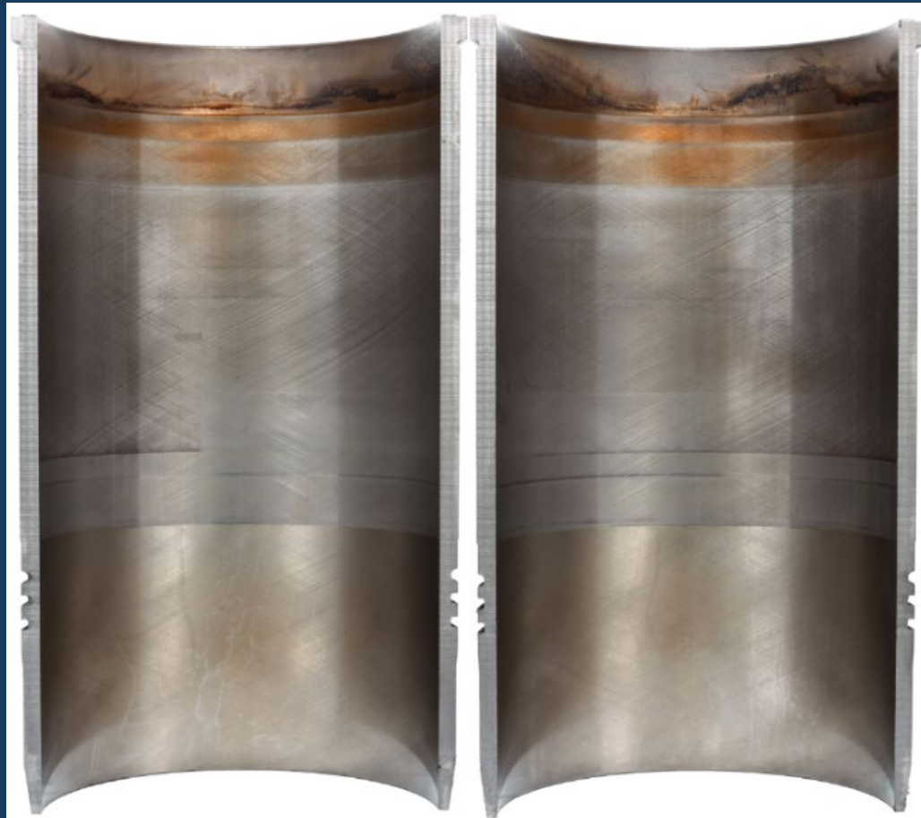
Anti-Thrust
